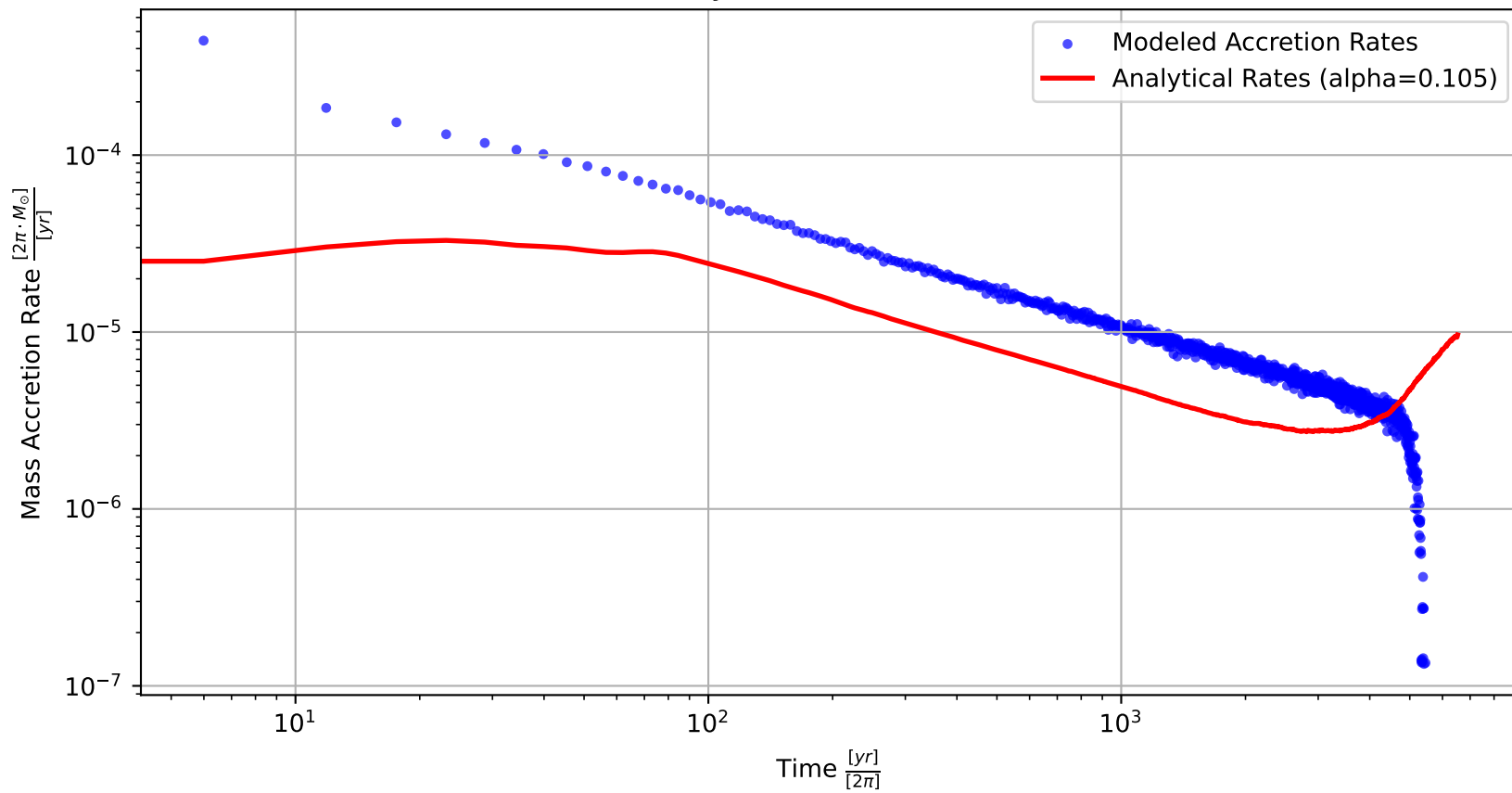
Modeled vs Analytical Accretion Rates (beta=2 \pi )
